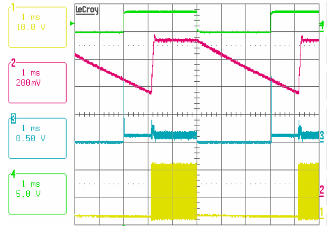
FIGURE 37. PRE-CHARGED START UP, V_{IN} = 19V , VID = 0.95V , Ch1: PHASE1, Ch2: V_O , Ch3: IMON, Ch4: VR_ON
